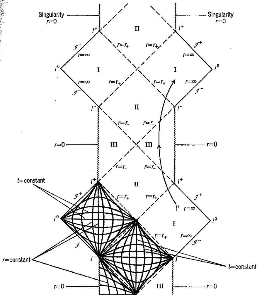
Fig. 18.6 Penrose diagram for maximal analytic extension ( e^2 < m^2 ).
