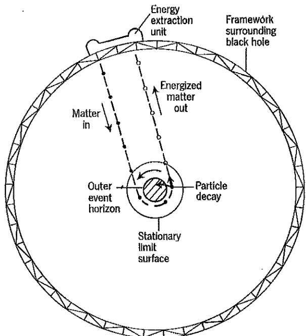
Fig. 19.10 Living off a rotating black hole.
