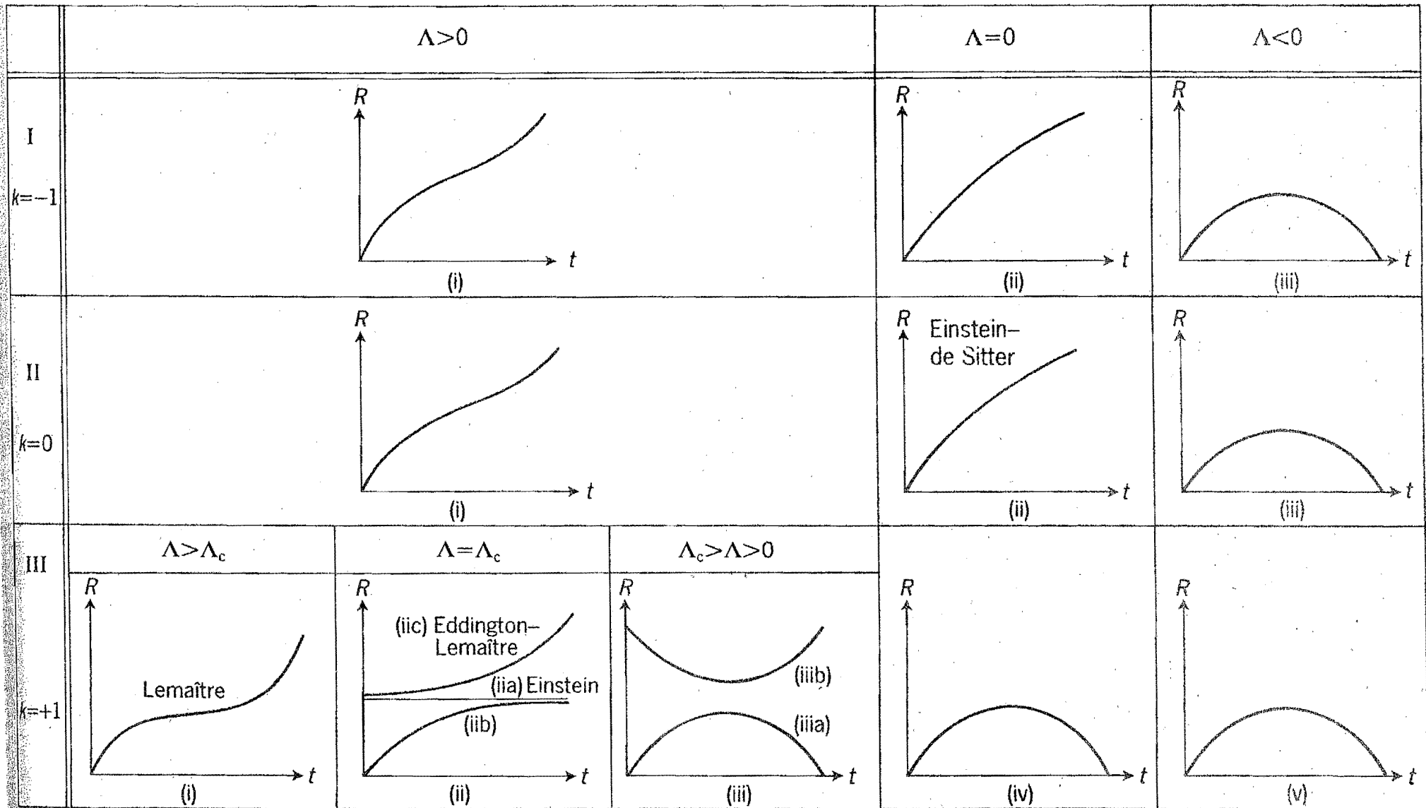
Fig. 23.1 Classification of Friedmann models.
