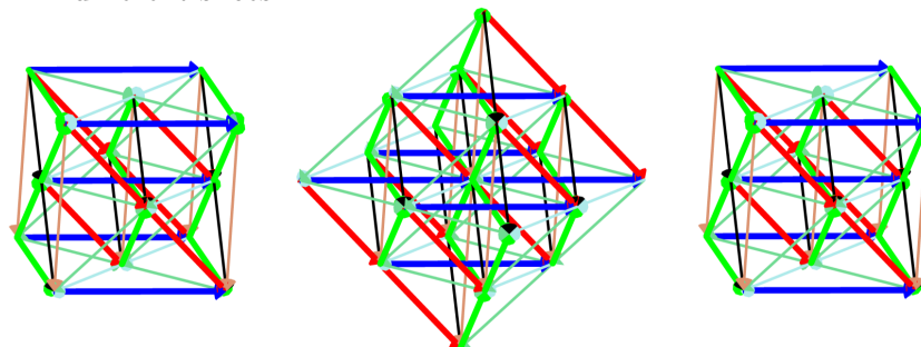
FIGURE 21. Slicing of F_4 using roots r^2 (red), r^3 (blue), and r^4 (green). Grey colored struts connect vertices from different slices.
