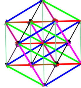
FIGURE 15. G_2 \subset B_3 = so(7)
