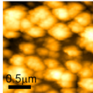
NSOM fluorescence
