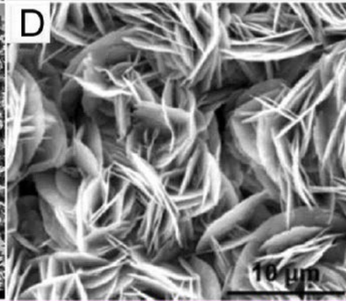
nanosheets
