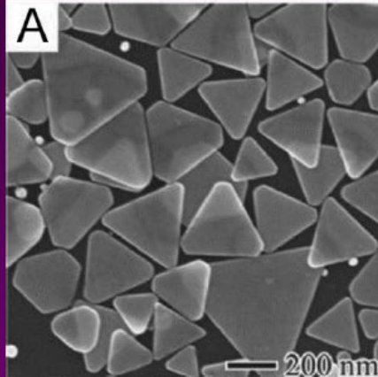
nanoprisms
