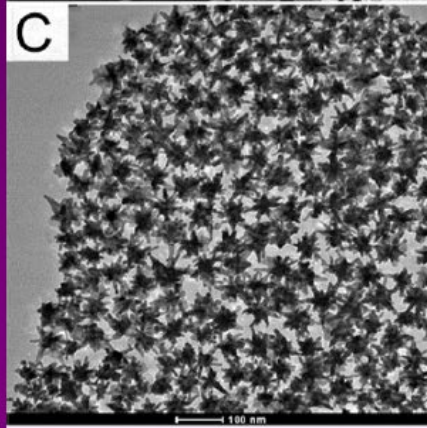
nanostars
