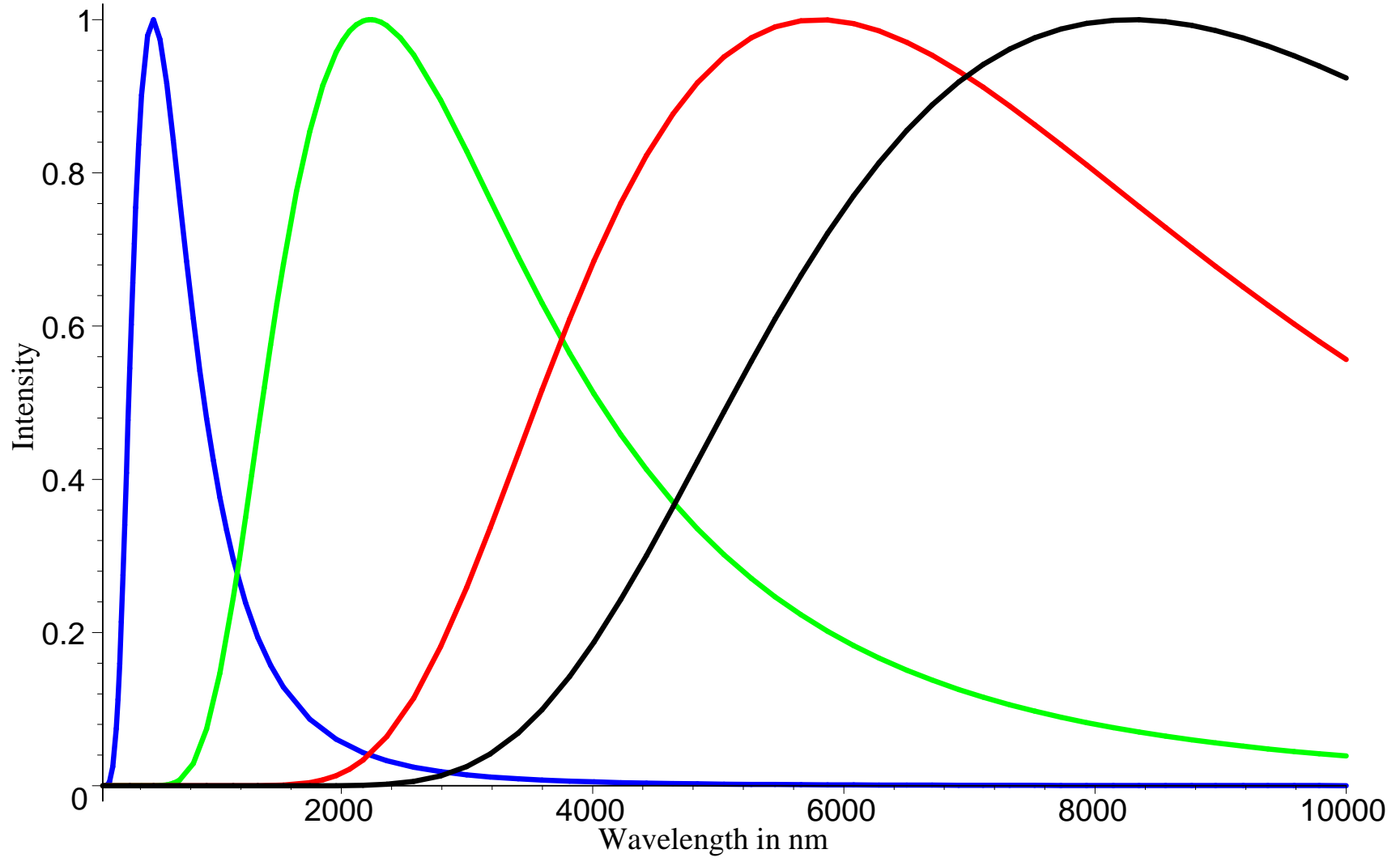
Planck Black Body Radiation Spectra For 5800, 1300, 500, 350 Kelvin
