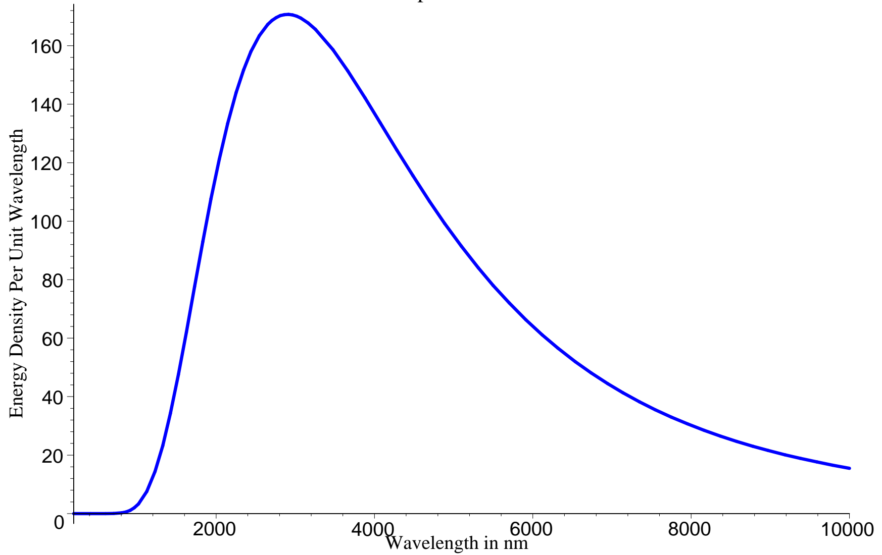
Planck Radiation Spectrum for 1000 Kelvin
