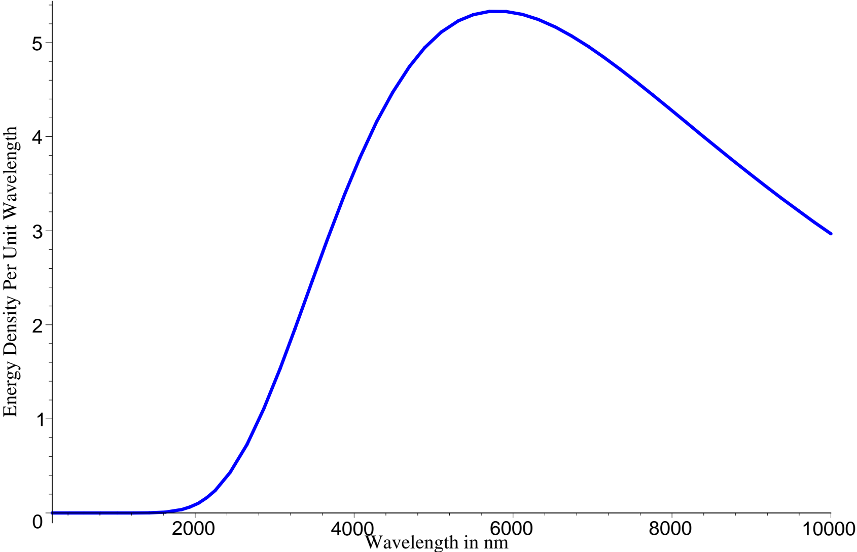
Planck Radiation Spectrum for 500 Kelvin
