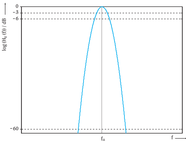
Fig. 4-8 Voltage transfer function of Gaussian filter in logarithmic level scale
