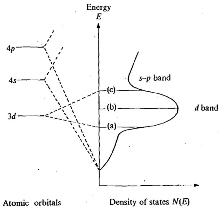
Fig. 3.13 Density of states resulting from the overlap of 3d, 4s and 4p atomic orbitals in a first-row transition metal. The Fermi level is indicated for elements: (a) early; (b) in the middle, and (c) late in the series.
