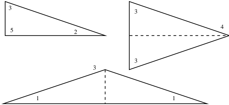
FIGURE 4. Case of n=5 : \mathcal{T}(2, 3, 5) , \mathcal{T}(4, 3, 3) and \mathcal{T}(1, 1, 3)
