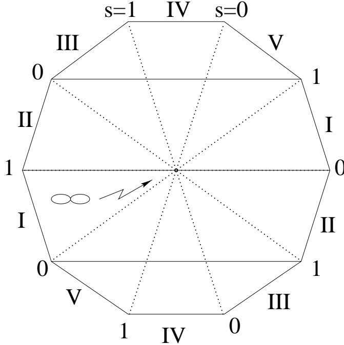
FIGURE 1. Case of j = 2 : X(2, 2, 1) ; horizontal cylinders marked.
