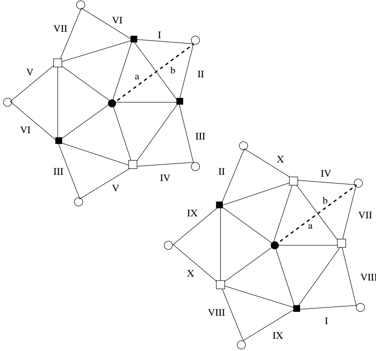
FIGURE 3. X(3, 3, 4) tiled by \mathcal{T}(3, 3, 4) .
