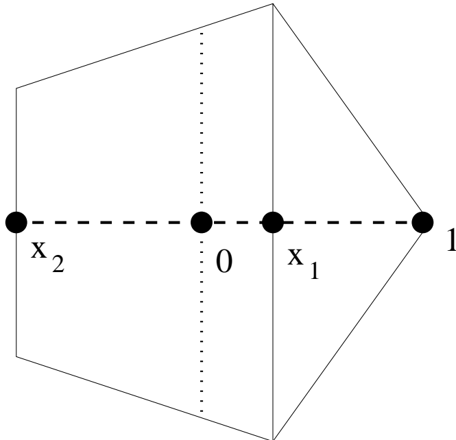
FIGURE 2. Case of n=5 : a single regular pentagon, with vertical cylinders and center marked.
