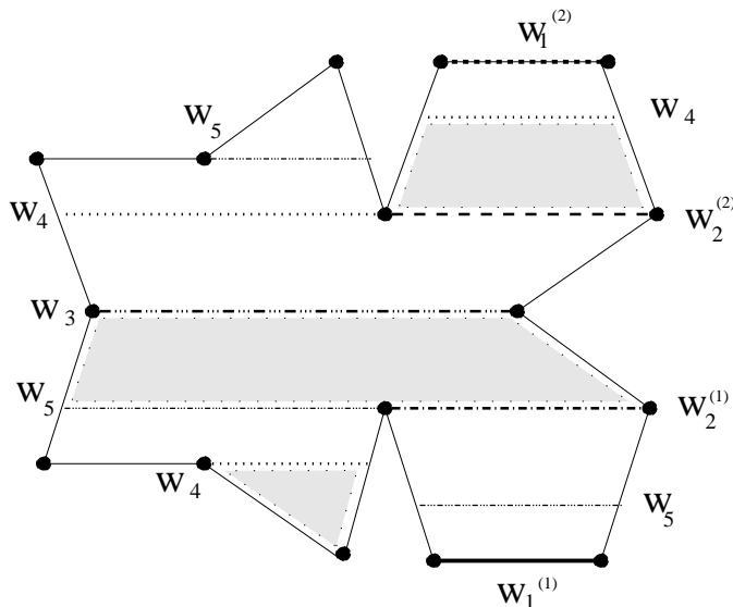
FIGURE 5. X(3, 5, 7) , the horizontal connections. \mathcal{N}(\mathcal{P}, \theta') = (2, 2, 1, 2) .
