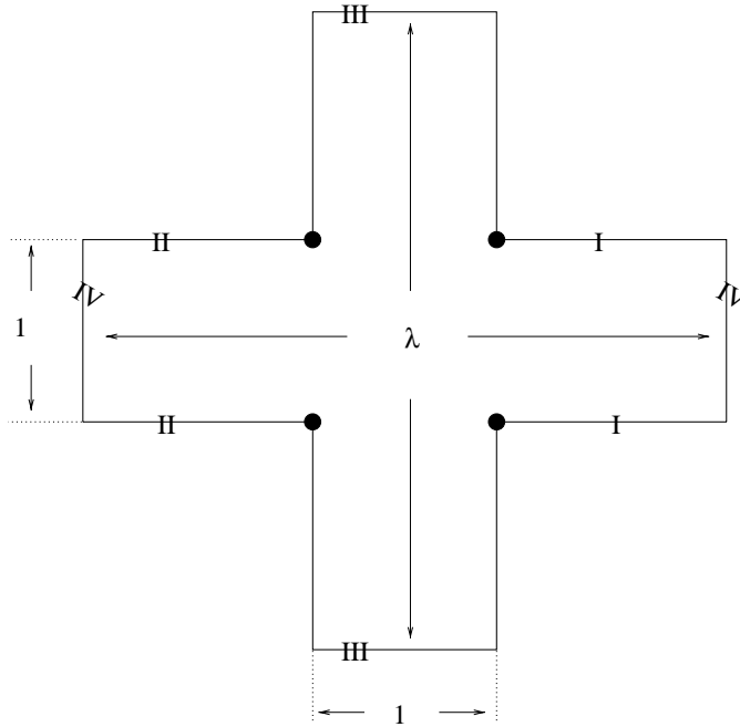
FIGURE 1. The cross of translation \lambda
