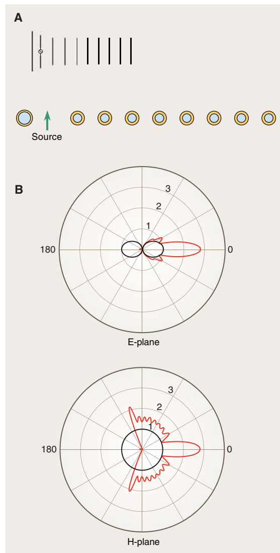
Fig. 3. Metananocircuit as a tool in the design of optical Yagi-Uda nanoantennas (30). (A) A sketch of conventional Yagi-Uda RF antenna is shown above. The collection of shell particles (with two different ratios of radii) around an optical point dipole source (e.g., a molecule) can form Yagi-Uda-type optical nanoarrays. (B) The theoretically evaluated radiation patterns of the optical Yagi-Uda-like nanoarrays in (A) at 620 nm (red), compared with that of a dipole alone (black). In (30), we used the core of SiO 2 and the shell of Ag in our analysis, with outer radius of 0.2\lambda_0 and ratios of radii of 0.851 and 0.834 for the left and right nanoshells, respectively. The distance between the left nanoshell and the source is 0.25\lambda_0 , while that on the right (and between the right particles) is 0.65\lambda_0 . [From (30)].
