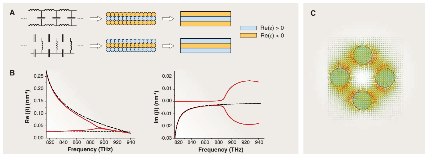
Fig. 4. Optical nanotransmission line based on the mn-circuits. (A) The concept of transmission lines in RF and microwave (left) can be brought into the optical domain using the notion of lumped nanocircuit elements (middle and right). By replacing the lumped inductor and capacitor with plasmonic [Re(ε) < 0] and dielectric [Re(ε) > 0] nanoparticles, respectively, the structures shown in the middle panel can be obtained. In the limit, when these nanoparticles merge into each other, the guided-wave structures sketched on the right are the result. These structures thus indeed function as optical nanotransmission (37). (B) The dispersion diagram of the waveguide shown in (A), when the SiO 2 and
