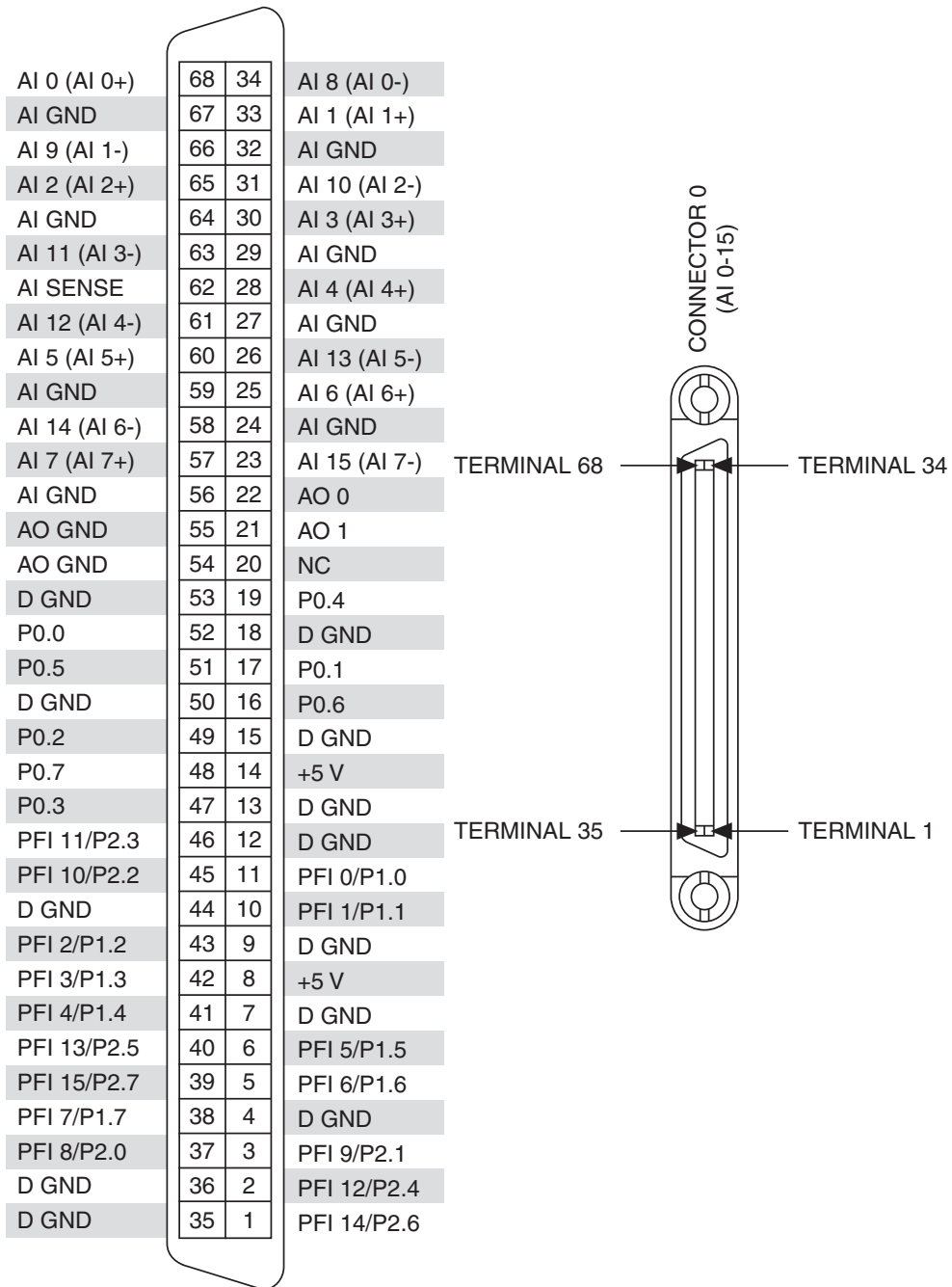
Figure A-2. PCI/PXI-6221 Pinout
