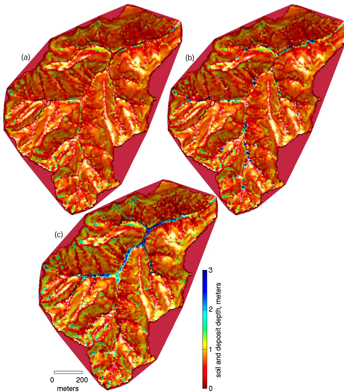
Plate 1. Shaded relief maps colored according to soil or sediment depth of (a) initial condition for model simulation, (b) after 200 years (18 years after the first fire), and (c) after 3000 years (the end of the simulation). The color scale is compressed to show variations in soil depth and to highlight all deposits greater than 3 meters in depth.
