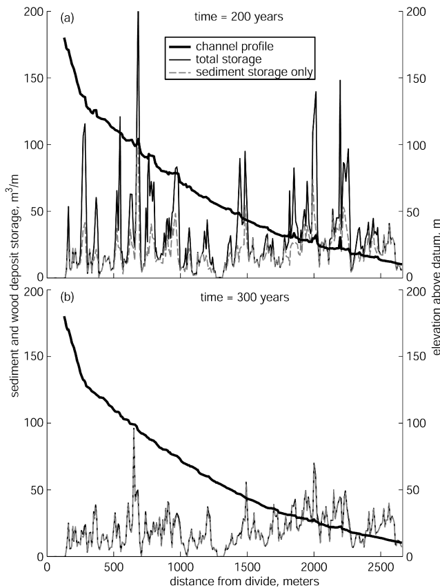
Figure 8. Simulated main channel profile and cross-sectional areas of sediment and wood deposit storage at every point along the main channel vs. distance downstream at two times, (a) 200 years (18 years after the first fire) and (b) 300 years (118 years after the first fire and before the second fire).
