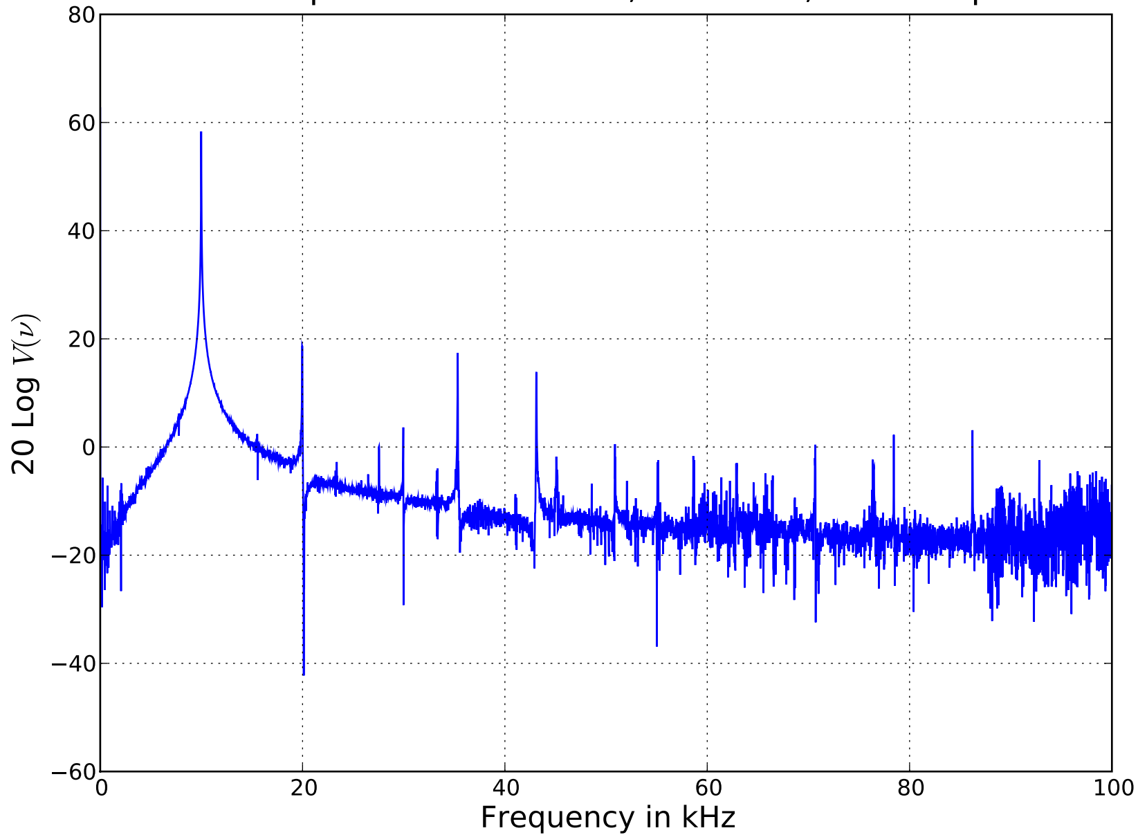
Power Spectrum: 2190 kHz, 200 kSPS, 10 kSamples
