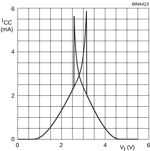
Fig.10 Typical AHC transfer characteristics; V_{CC} = 5.5 V.
