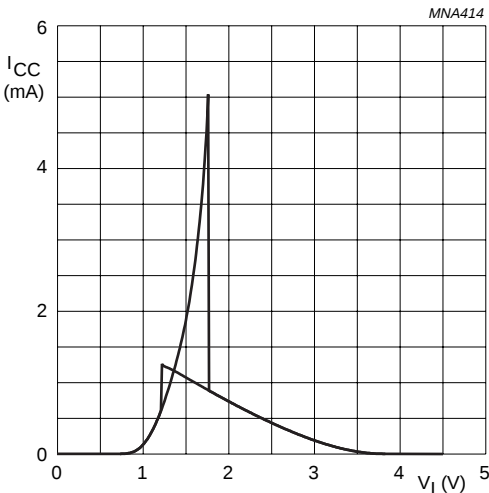
Fig.11 Typical AHCT transfer characteristics; V_{CC} = 4.5 V.
