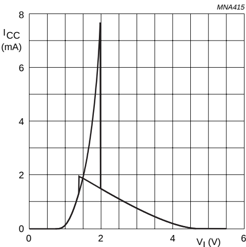
Fig.12 Typical AHCT transfer characteristics; V_{CC} = 5.5 V.
