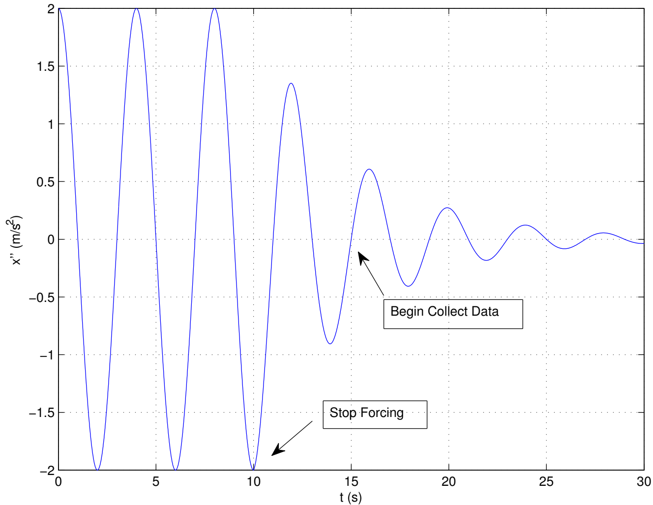
Accelerometer data
