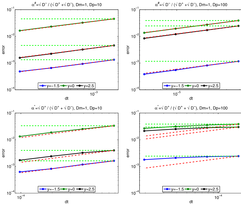
Fig. 2. Error for the SDE-BE method demonstrating half order convergence (the dashed and dash-dot lines indicate the zeroth and half order reference lines, respectively).
