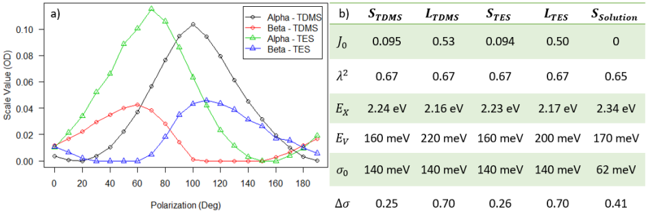
Figure 3: (a) Plot of the scaling factors \alpha and \beta used in the linear combination fits \alpha S + \beta L for TES and TDMS. (b) Fit parameters for S and L lineshapes for TES and TDMS as well as for the TES solution fit with progressive broadening.
